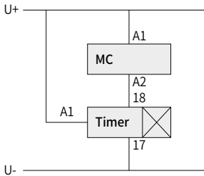
※ A1/A2 : Coil terminal, 17/18 : Timer terminal
