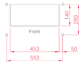
Panel cutting (Fixing hole)
