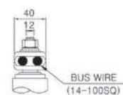
TERMINAL DETAIL
